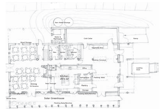
FIRST FLOOR PLAN Not to Scale
